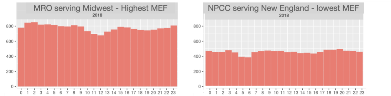
Figure 2: Hourly marginal emissions factors for MRO and NPCC, which serve parts of the Midwest and New England
