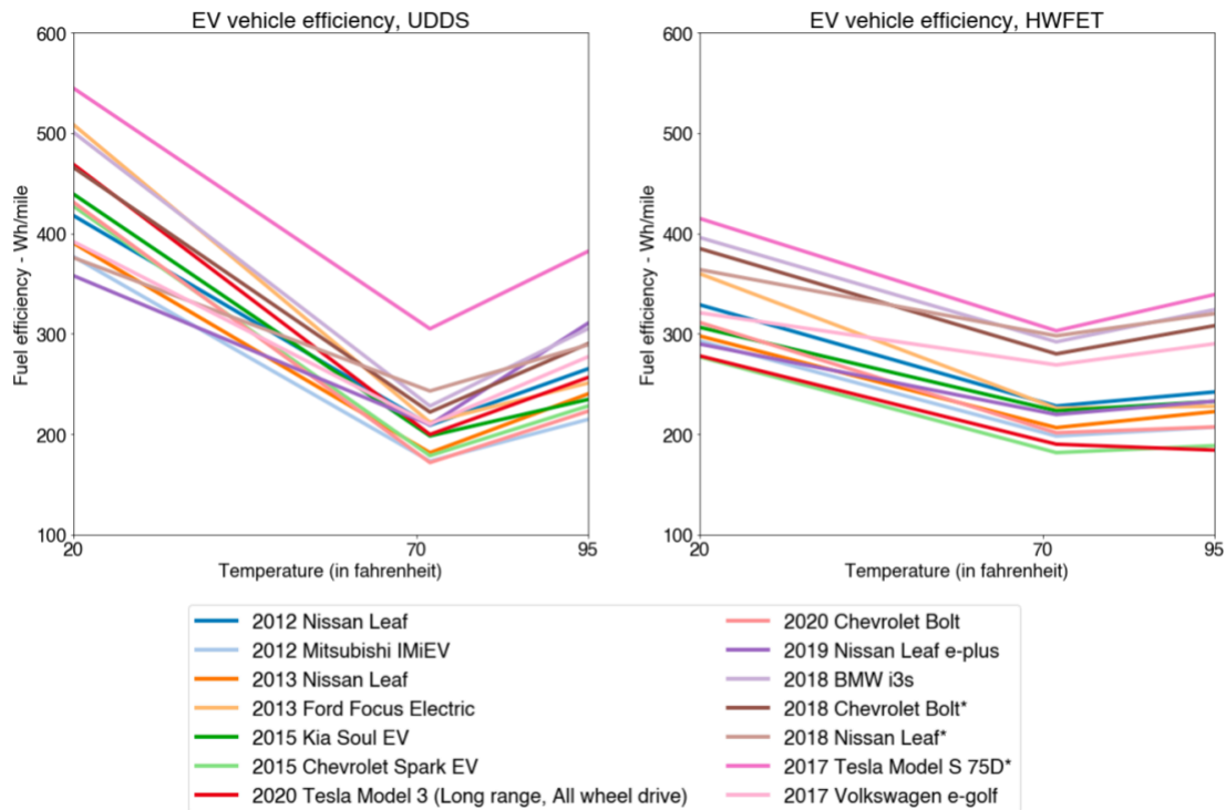
Figure 1: Electric vehicle fuel efficiency (Wh/mile) dependent on temperature and drive cycle.
